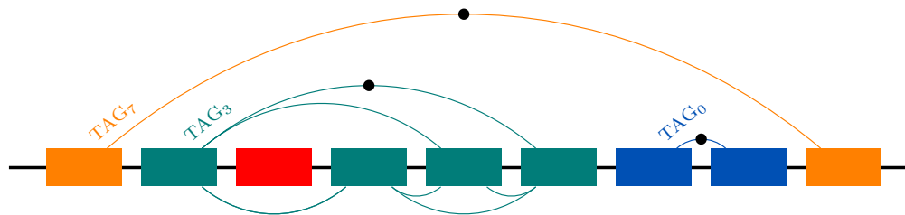
Figure 3.1. Schematic representation of TAG definitions. Several genes are represented on a linear chromosome. The red box represent a singleton gene. Orange boxes represent a TAG with two duplicate genes separated by 7 other genes ( TAG_7 ). Four green boxes constitute a TAG, the gene at the extremities are separated by three genes ( TAG_3 ). The two blue boxes represents a TAG with two genes next to each other ( TAG_0 ). The bended edges represents the homology links between each pair of genes within a TAG.
